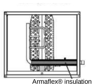
Figure 8 – Horizontal A-Coil w/ side connections
